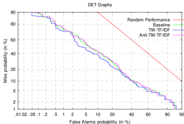
Figure 3. DET curves for TW-TF/IDF and Anti-TW-TF/IDF.
